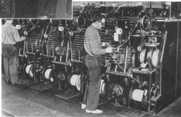
The insulated wires are twisted into pairs to form telephone circuits.
