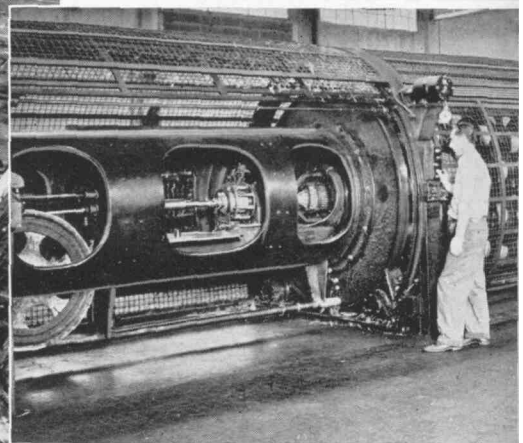
Twisted pairs of wire are combined in a stranding machine to form a cable.
